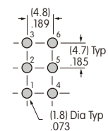
Double Pole
