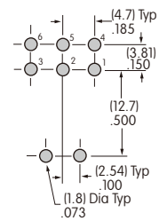
Double Pole
